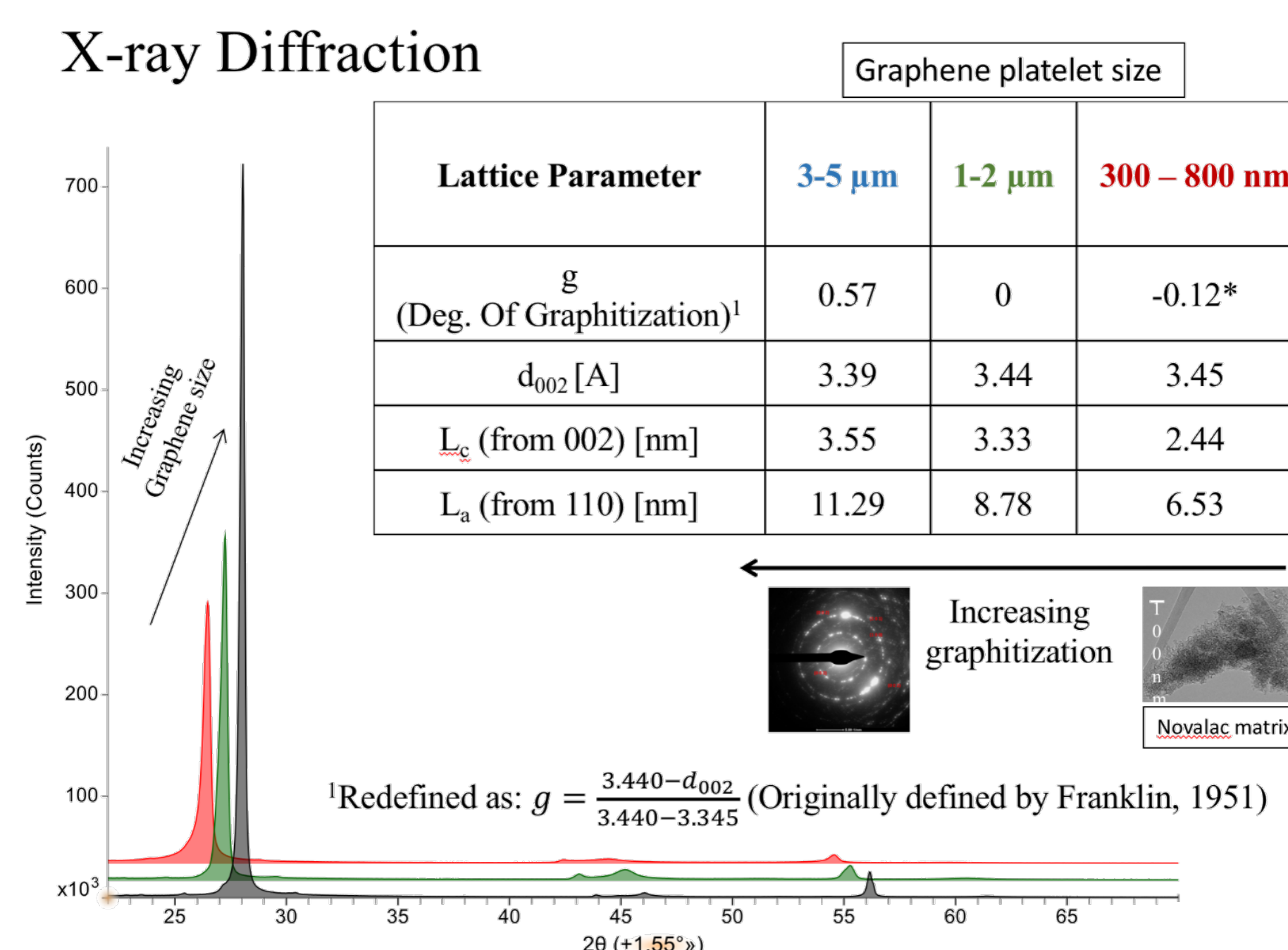
Carbon Graphitization
