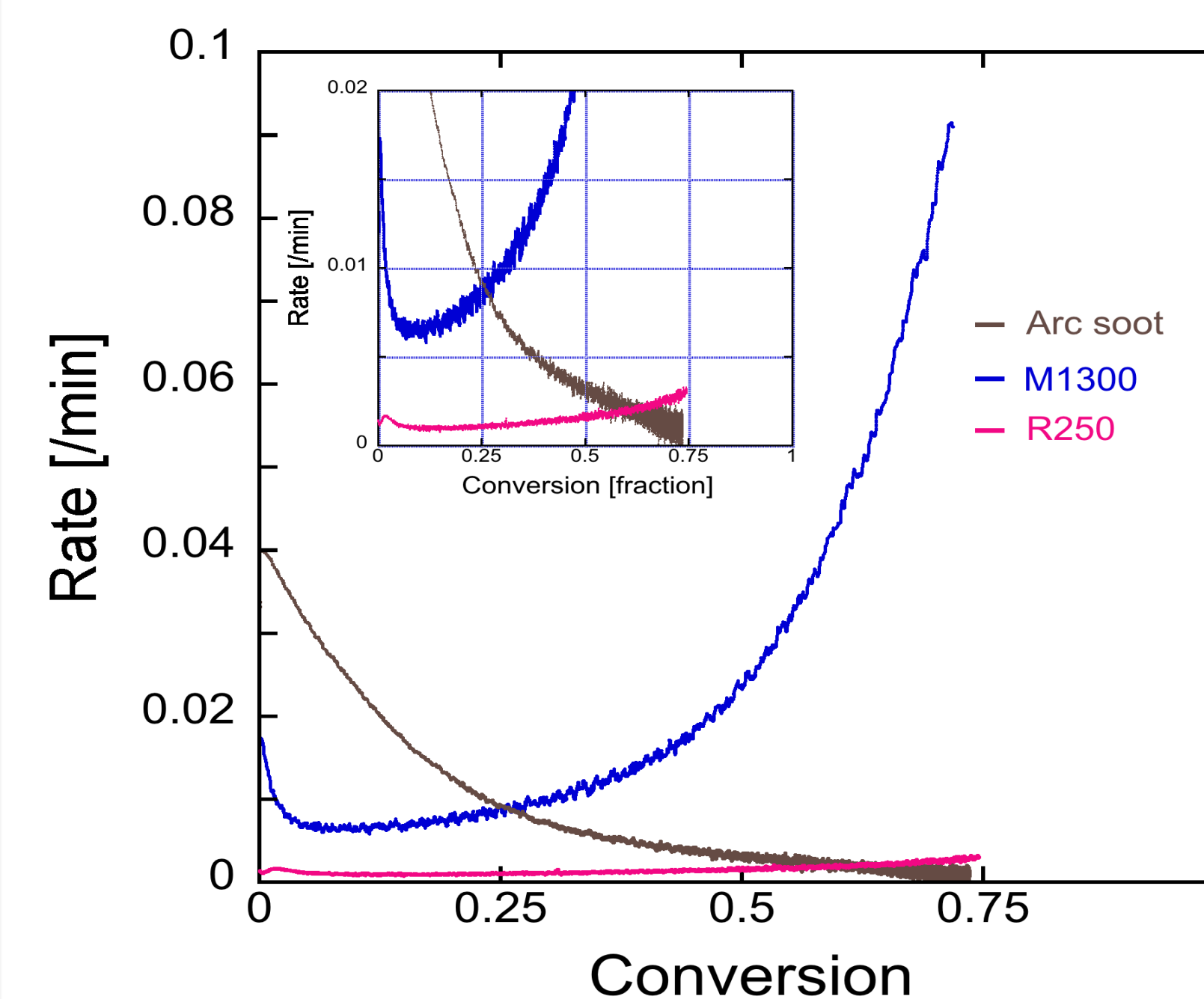
NanoStructure – Reactivity in Oxidation
