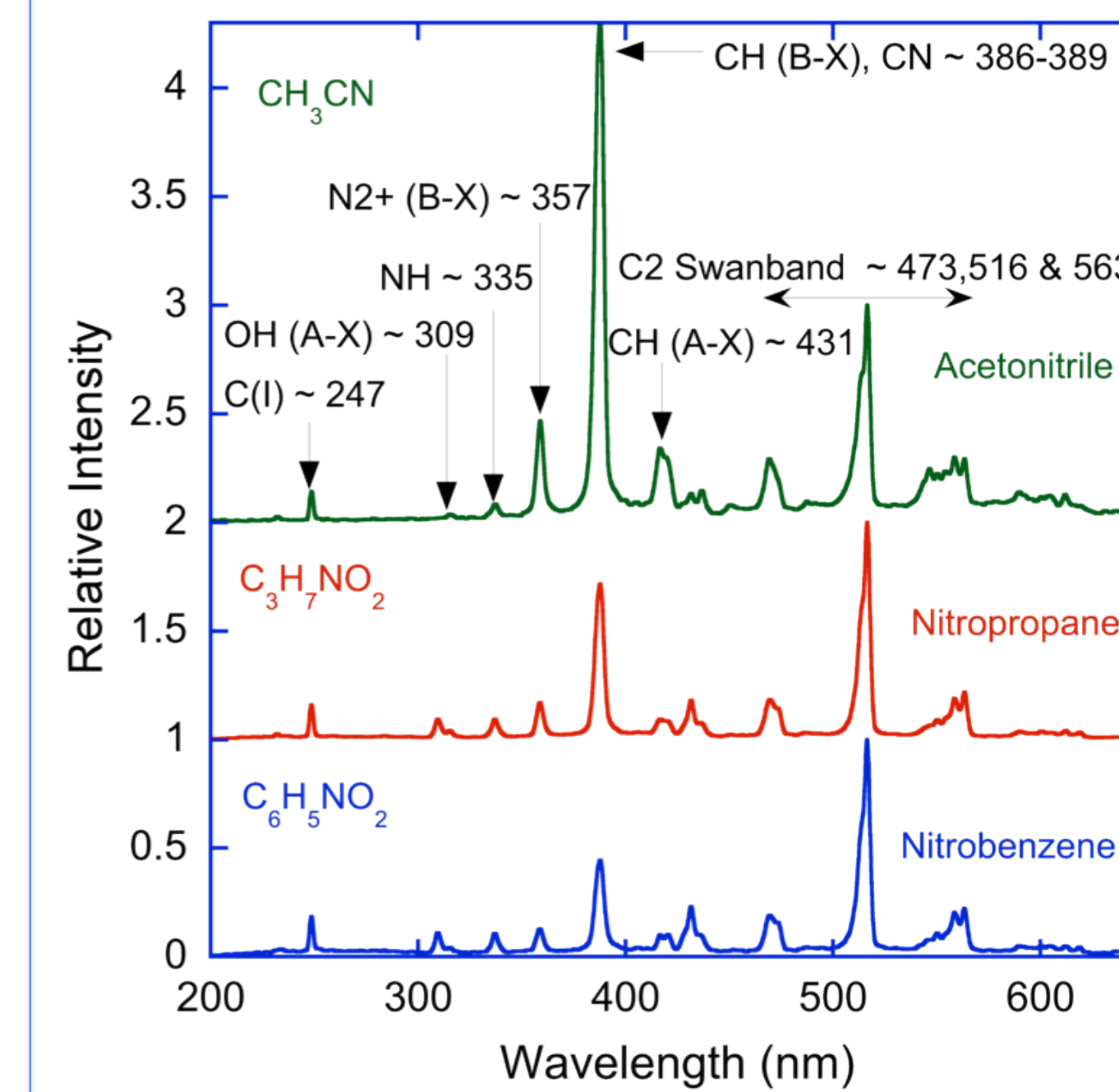
Plasma & Combustion Spectroscopic Diagnostics
