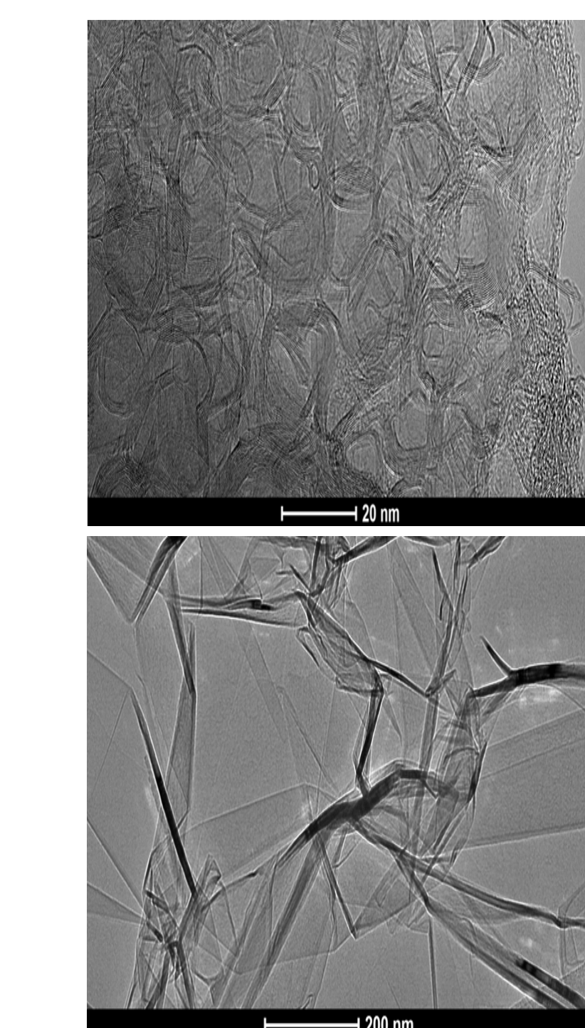
Carbon-carbon Composites
