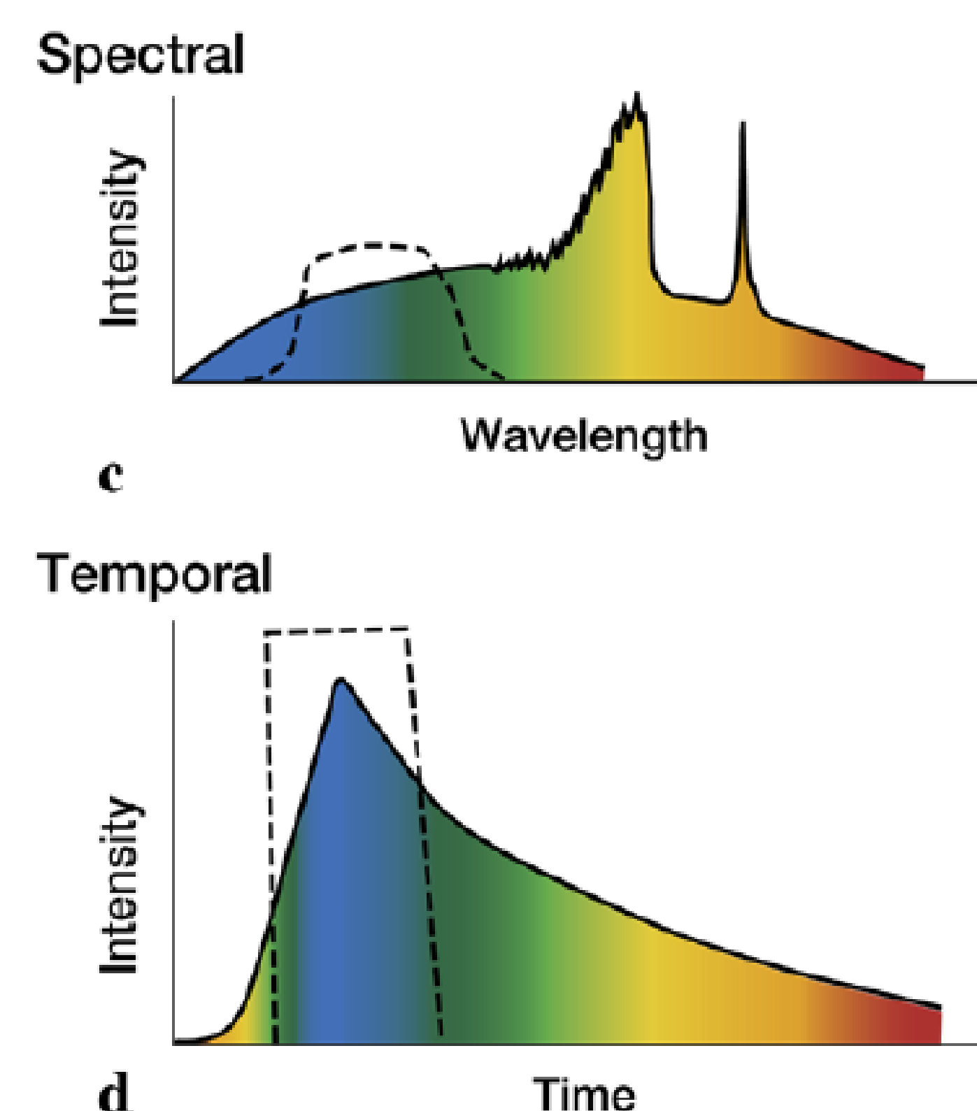
Laser-induced Incandescence (LII)
